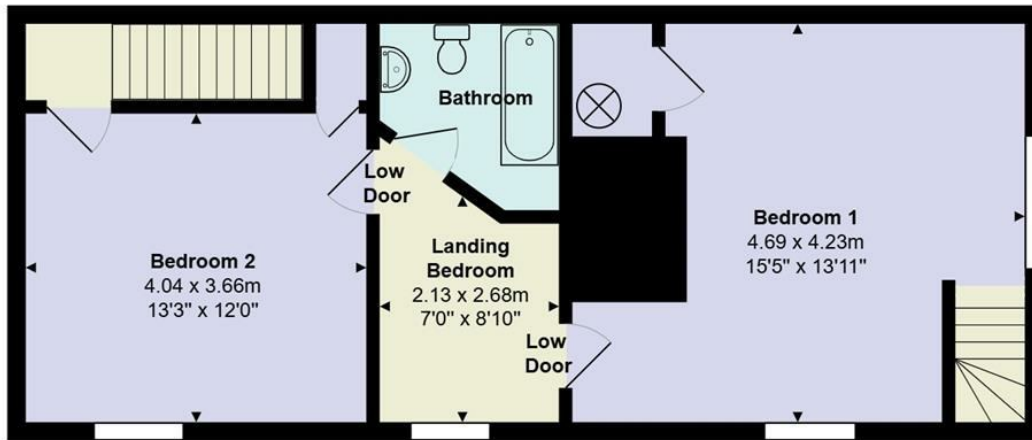
FIRST FLOOR
